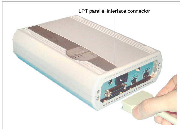
Figure 4.3 Connecting the LPT parallel interface cable (emulator PC7501 side)
