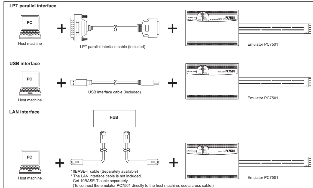
Figure 4.1 Outline for interface cable connections
