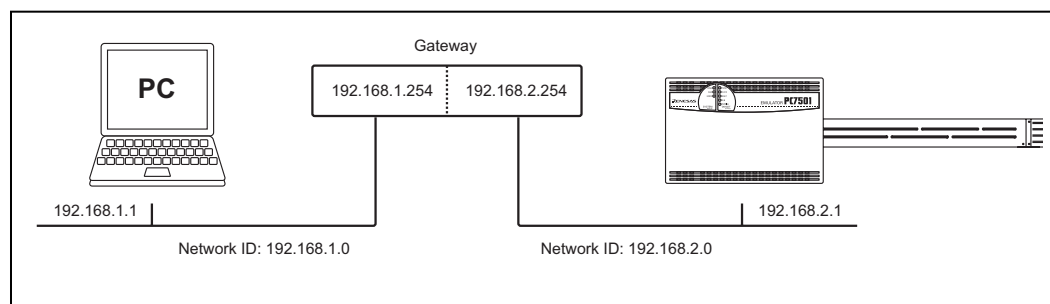
Figure 4.6 Network configuration
