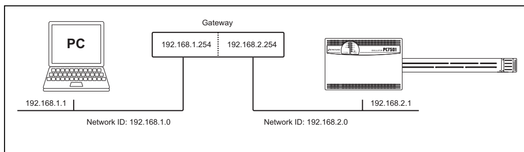
Figure 5.1 Network configuration
