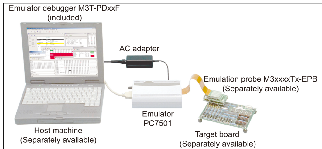
Figure 2.1 Emulator PC7501 system configuration
